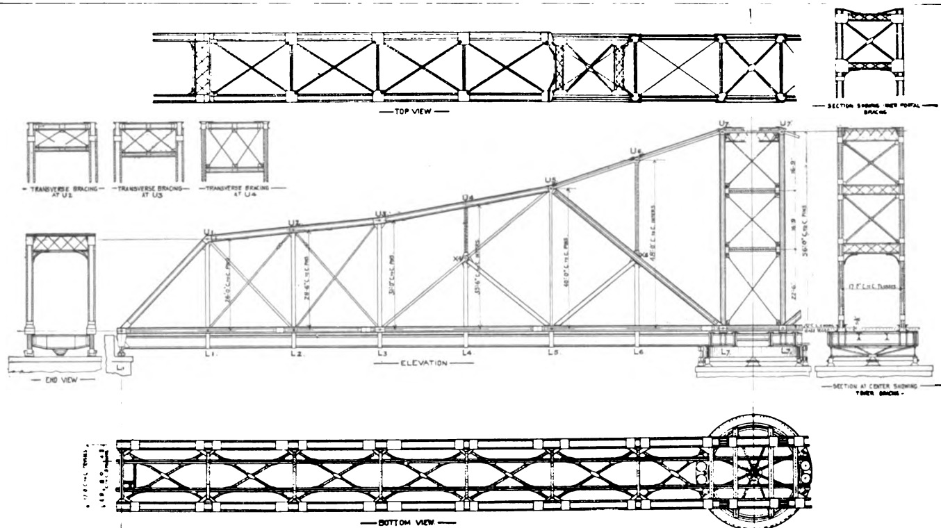
LACROSSE BRIDGE RENEWAL—DRAW SPAN OVER THE MAIN CHANNEL.
