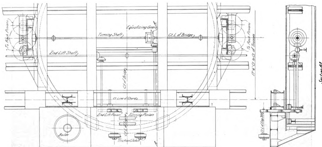
Plan of Machinery
